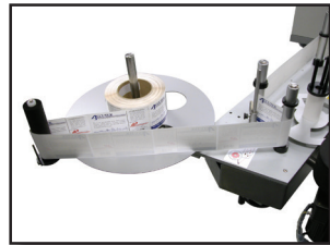
Feed wheel
